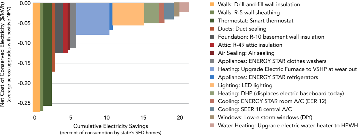
Figure 15. Electric Efficiency Supply Curve for Utah
