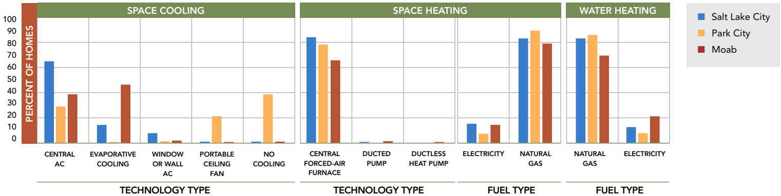
Figure 5: Residential Space Heating, Space Cooling, and Water Heating by Technology and Fuel Type
