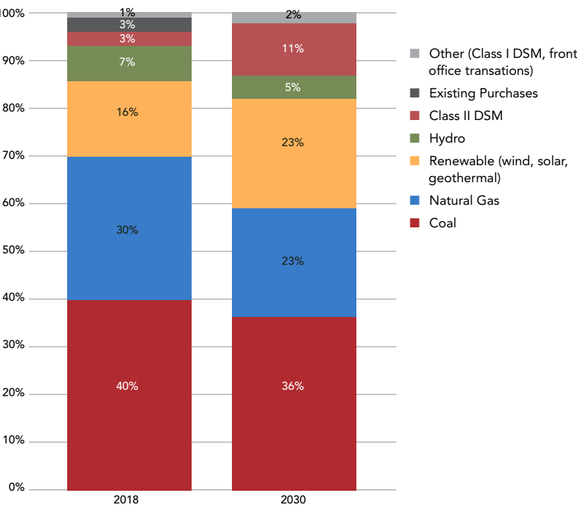
Figure 10. PacifiCorp System Energy Mix, 2018 and 2030
