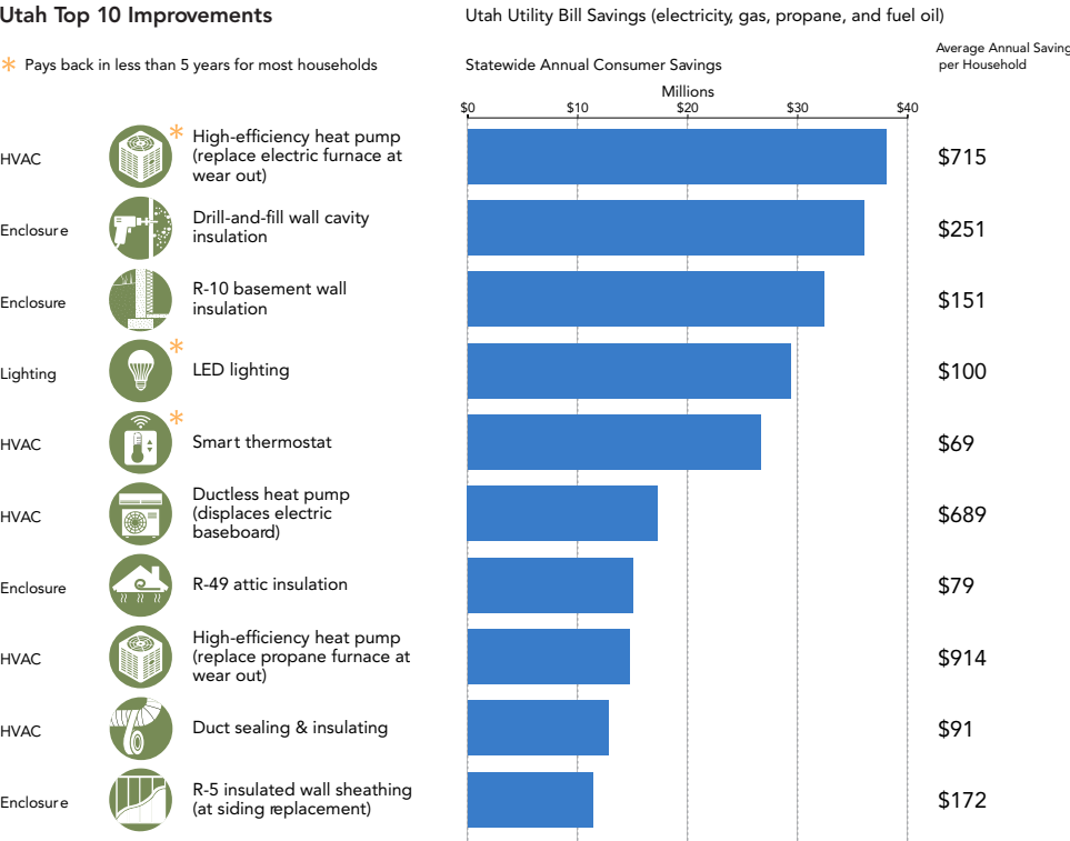
Figure 14. The Ten Largest Opportunities for Total Utility Bill Savings for Homeowners in Utah
