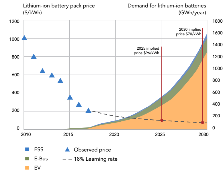
Figure 17. Lithium-ion Battery Pack Price Forecast
