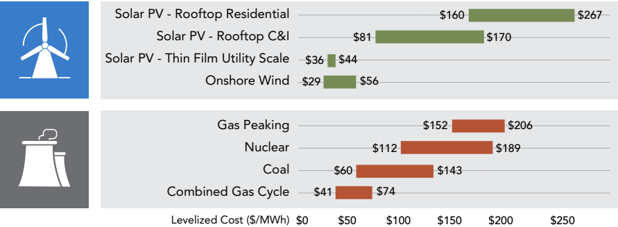
Figure 18. Levelized Cost of Utility Scale Renewable Energy Resources, Without Subsidies
